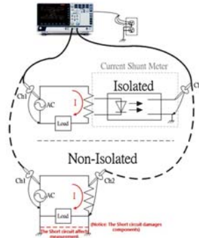
The measurement issue for Non-Isolated Shunt meter
